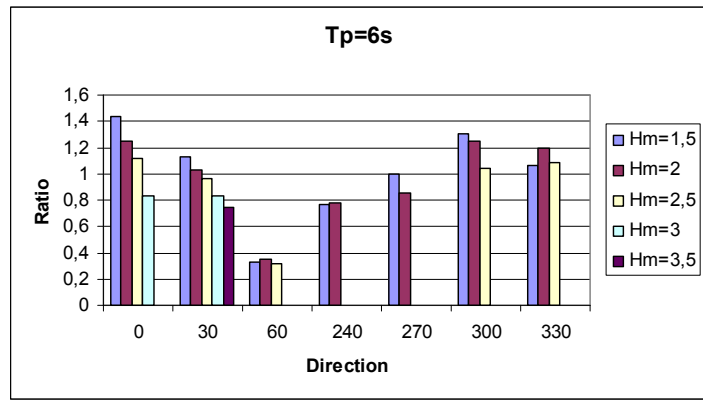
Figure 16: Hm0 near-shore/ Hm0 offshore (Tp=6 s)
