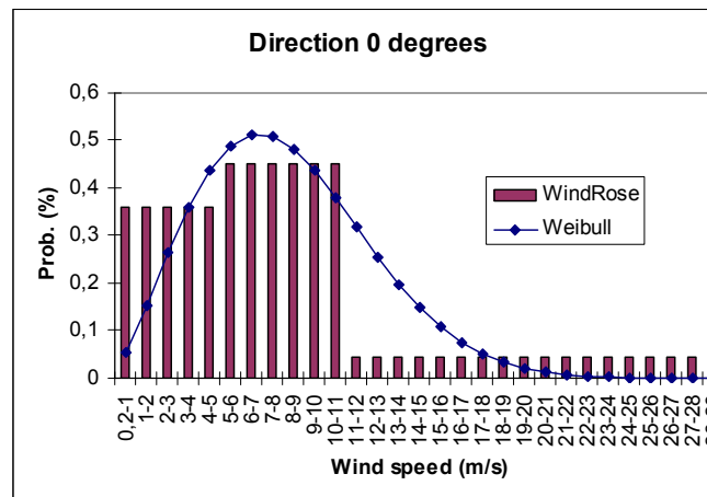
Figure 4: Weibull distribution deducted from the wind rose
