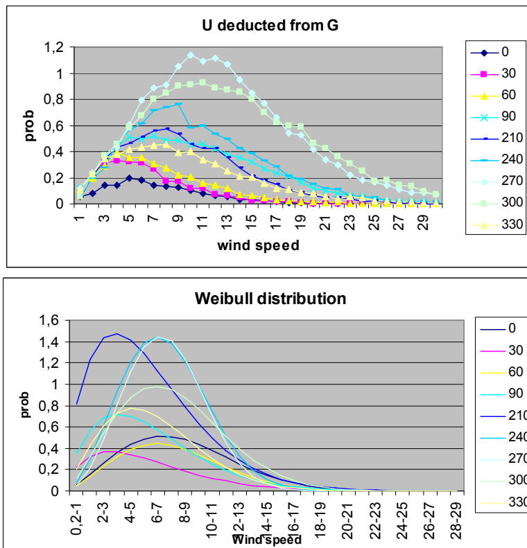
Figure 7: Comparison between the Weibull distribution and U deduced from G
