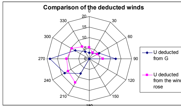
Figure 6: Comparison of the deduced winds (probabilities of occurrences)
