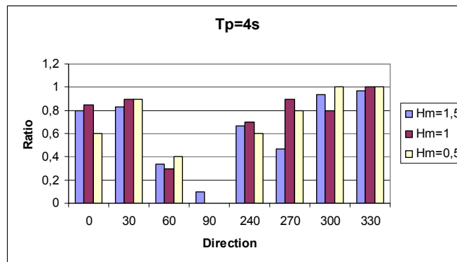
Figure 15: H_{m0} near-shore/ H_{m0} offshore ( T_p=4 s)
