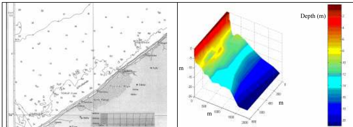
Figure 12 : modelling of the bathymetry
