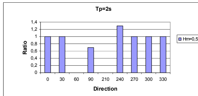
Figure 14: H_{m0} near-shore/ H_{m0} offshore ( T_p=2 s)
