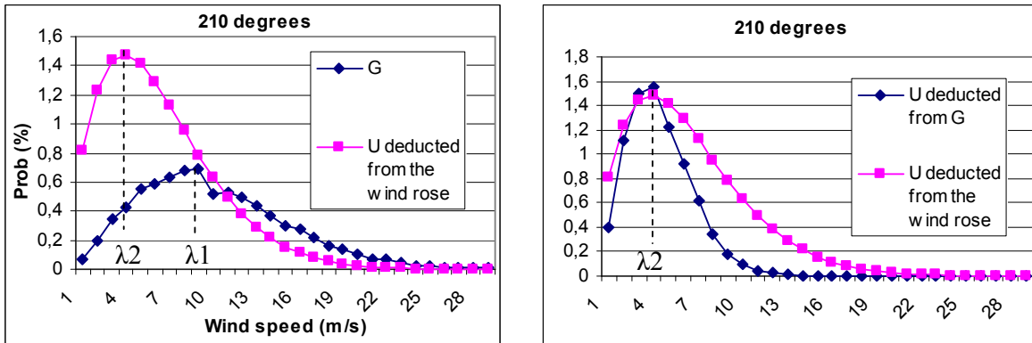
Figure 8 : Results of the conversion geostrophic wind/ground wind
