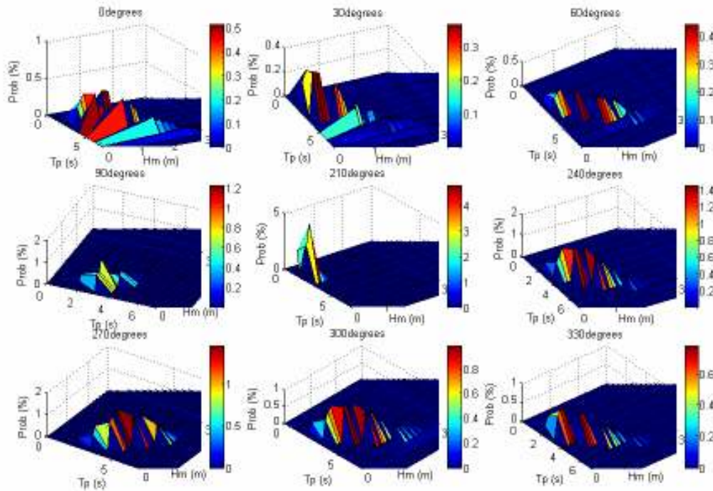
Figure 9 : Deducted offshore sea states per direction
