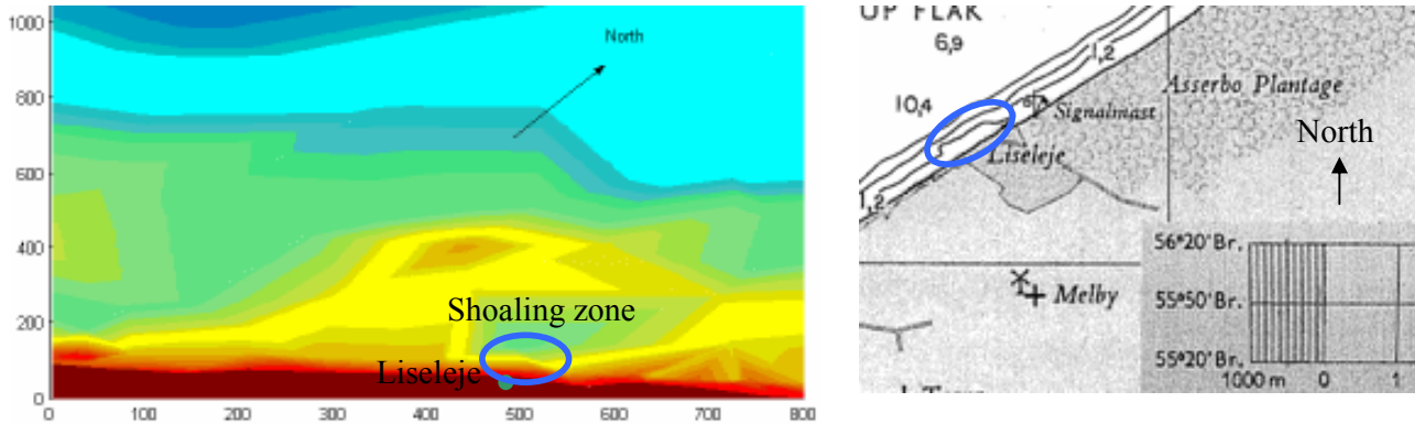
Figure 17 : Shoaling zone at Liseleje
