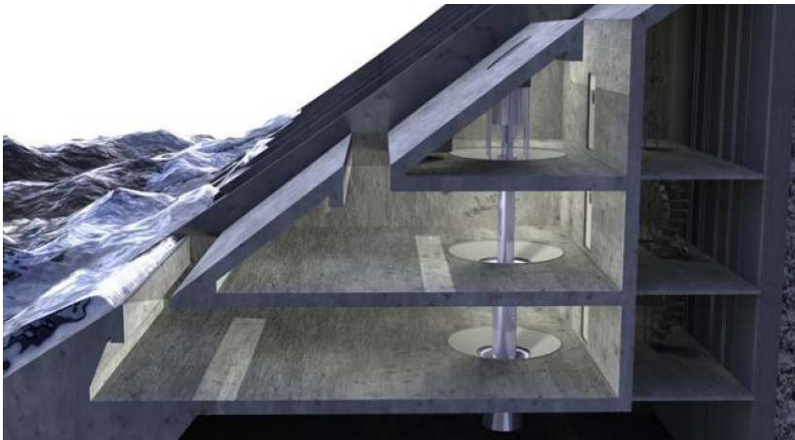
Figure 1. Artistic drawing of the SSG concept. 3-level reservoir and multistage turbine (WaveEnergy AS).
